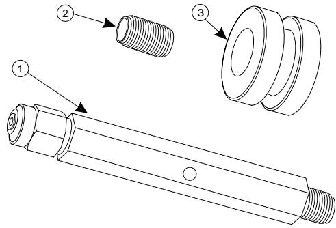
Figure 1. Model 01-118 Cable Assembly Tool
