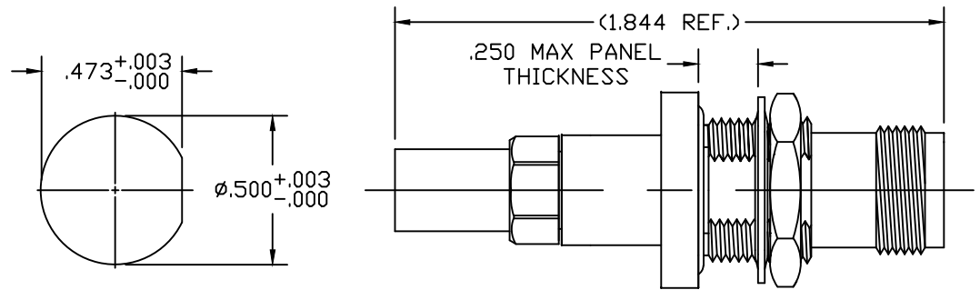
RECOMMENDED MOUNTING HOLE
